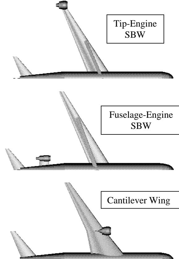
Figure 4. Minimum TOGW Designs.
