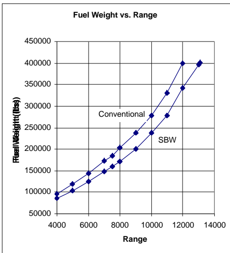
Figure 7. Effect of Range on Fuel Weight.
