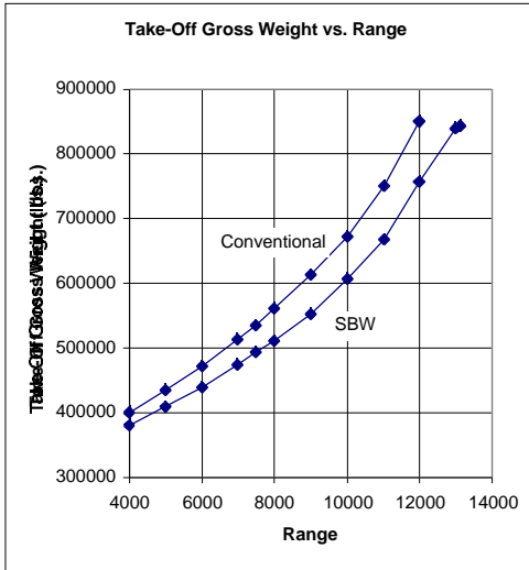
Figure 6. Effect of Range on TOGW.
