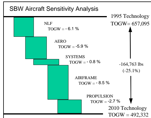
Figure 9. SBW Technology Sensitivity Analysis.
