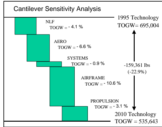
Figure 8. Cantilever Technology Sensitivity Analysis.
