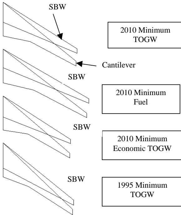
Figure 5. Optimum Cantilever and SBW Designs.
