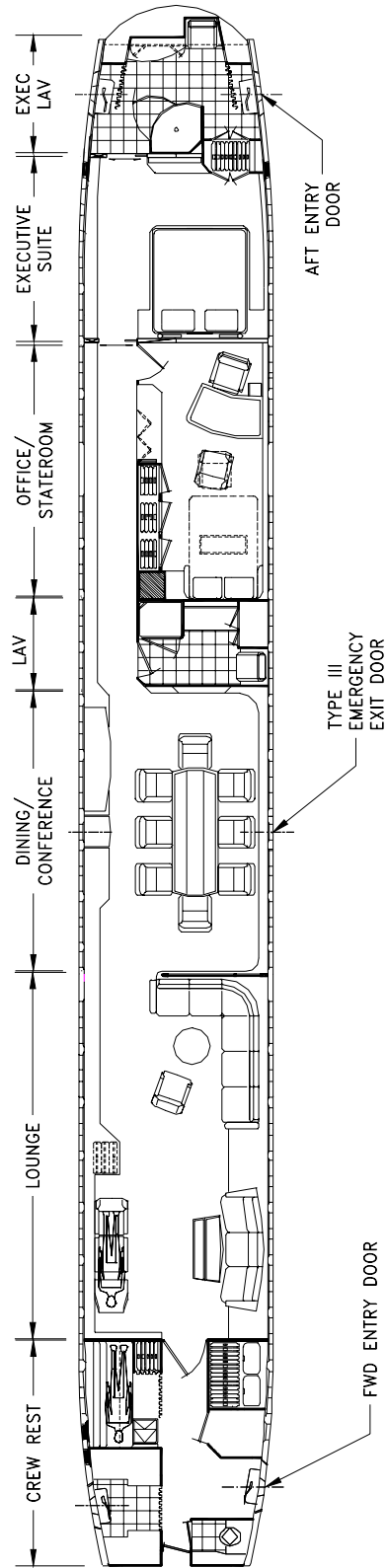
TYPICAL 737 BBJ2 INTERIOR ARRANGEMENT
