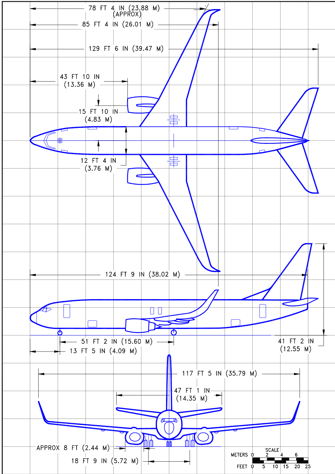
2.2.12 GENERAL DIMENSIONS MODEL 737-800 WITH WINGLETS, 737 BBJ2
