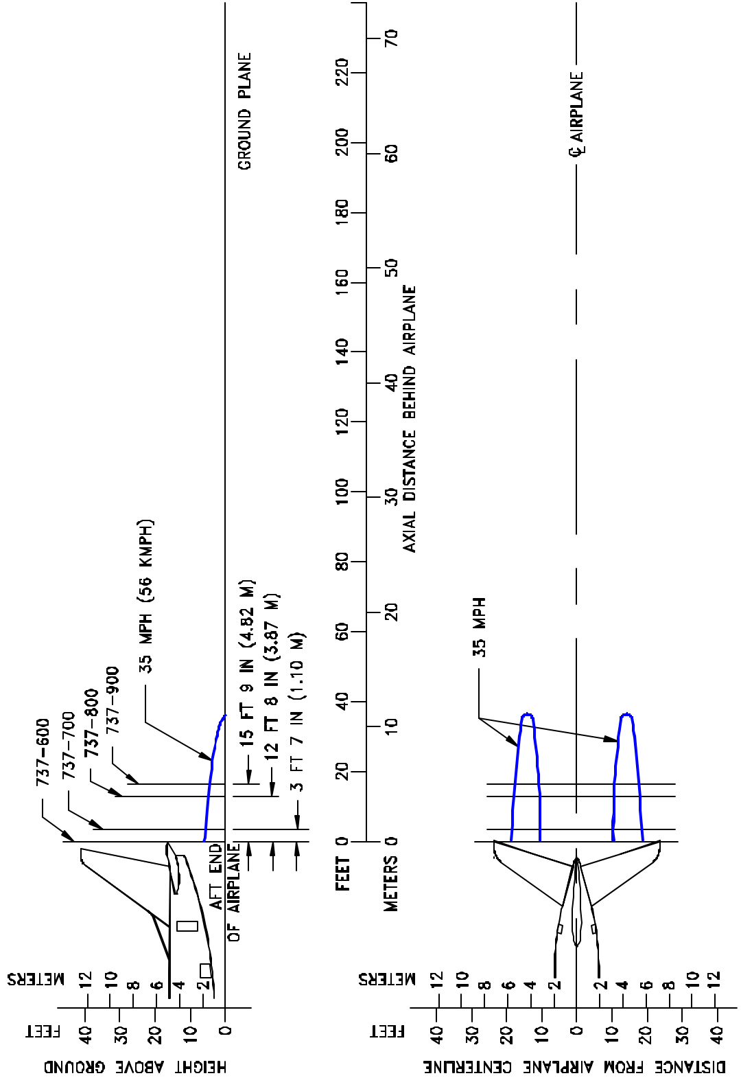
6.1.3 PREDICTED JET ENGINE EXHAUST VELOCITY CONTOURS - IDLE THRUST MODEL 737-600, -700, -800, -900, ALL MODELS
