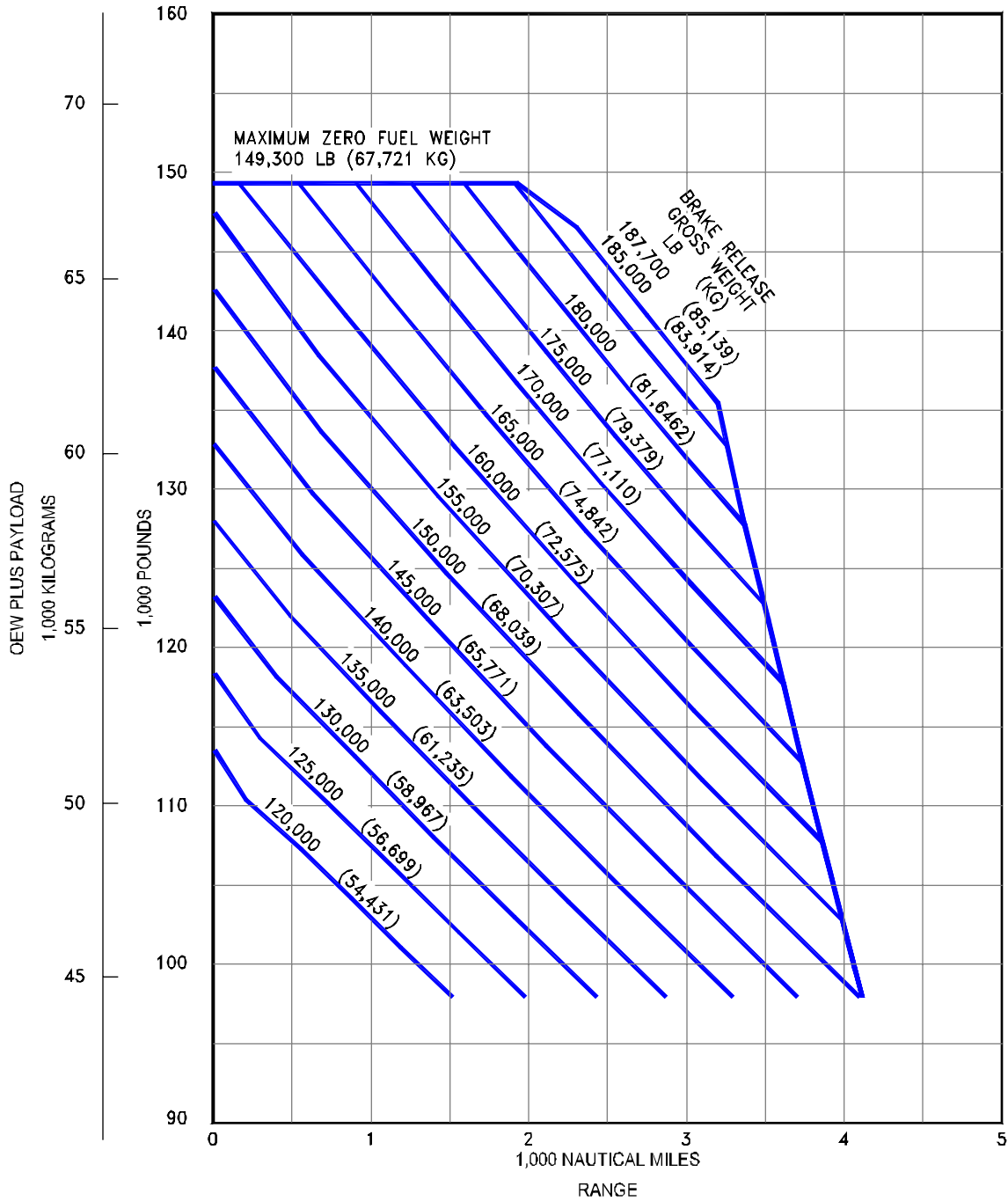
3.2.19 PAYLOAD/RANGE FOR LONG-RANGE CRUISE MODEL 737-900ER WITH WINGLETS
