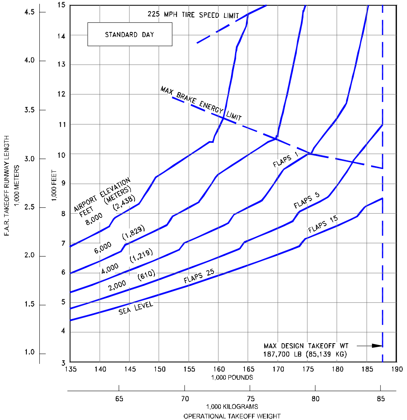
3.3.151 F.A.R. TAKEOFF RUNWAY LENGTH REQUIREMENTS STANDARD DAY, DRY RUNWAY MODEL 737-900ER (CFM56-7B27/3B1F ENGINES AT 27,300 LB SLST)
