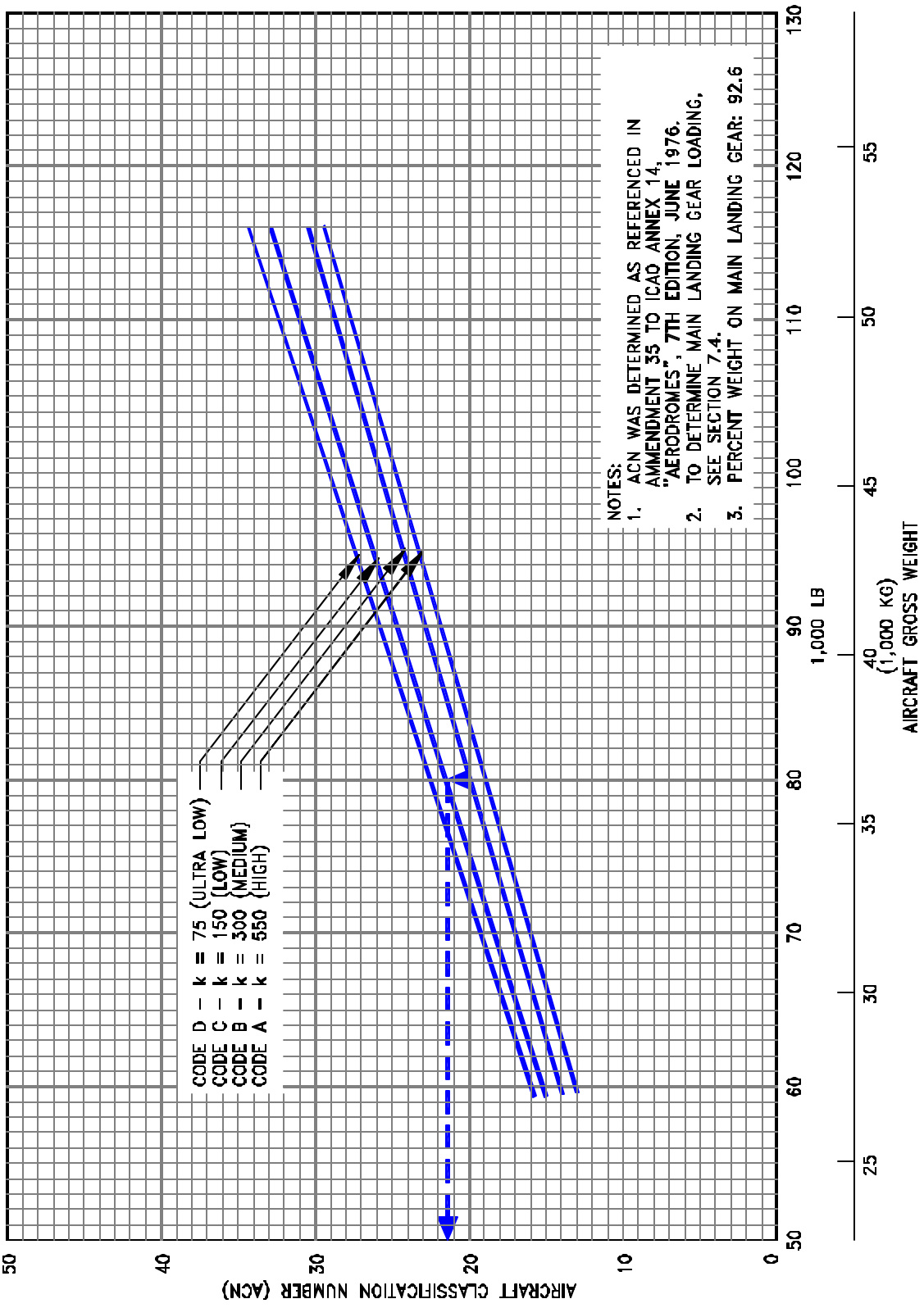
7.10.21 AIRCRAFT CLASSIFICATION NUMBER - RIGID PAVEMENT MODEL 737-100, -200, ADV 737-200 AT 110,000 TO 117,500 LB (49,900 TO 53,290 KG) MTW
